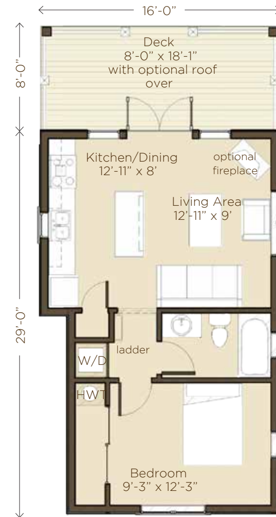
Main floor
